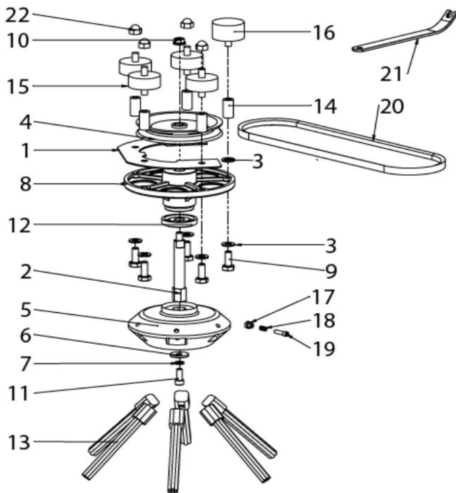
Brush Head, Spindel, Belt
